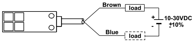
WIRING DIAGRAM
